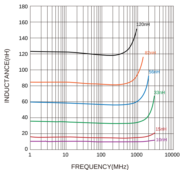
Inductance VS. Frequency Characteristics:
