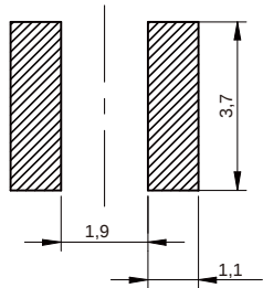
Land Pattern: [mm]
