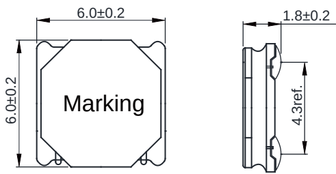
Dimensions: [mm]
