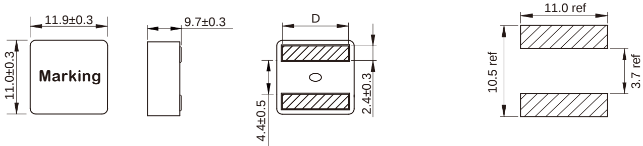
Land Pattern: [mm]
